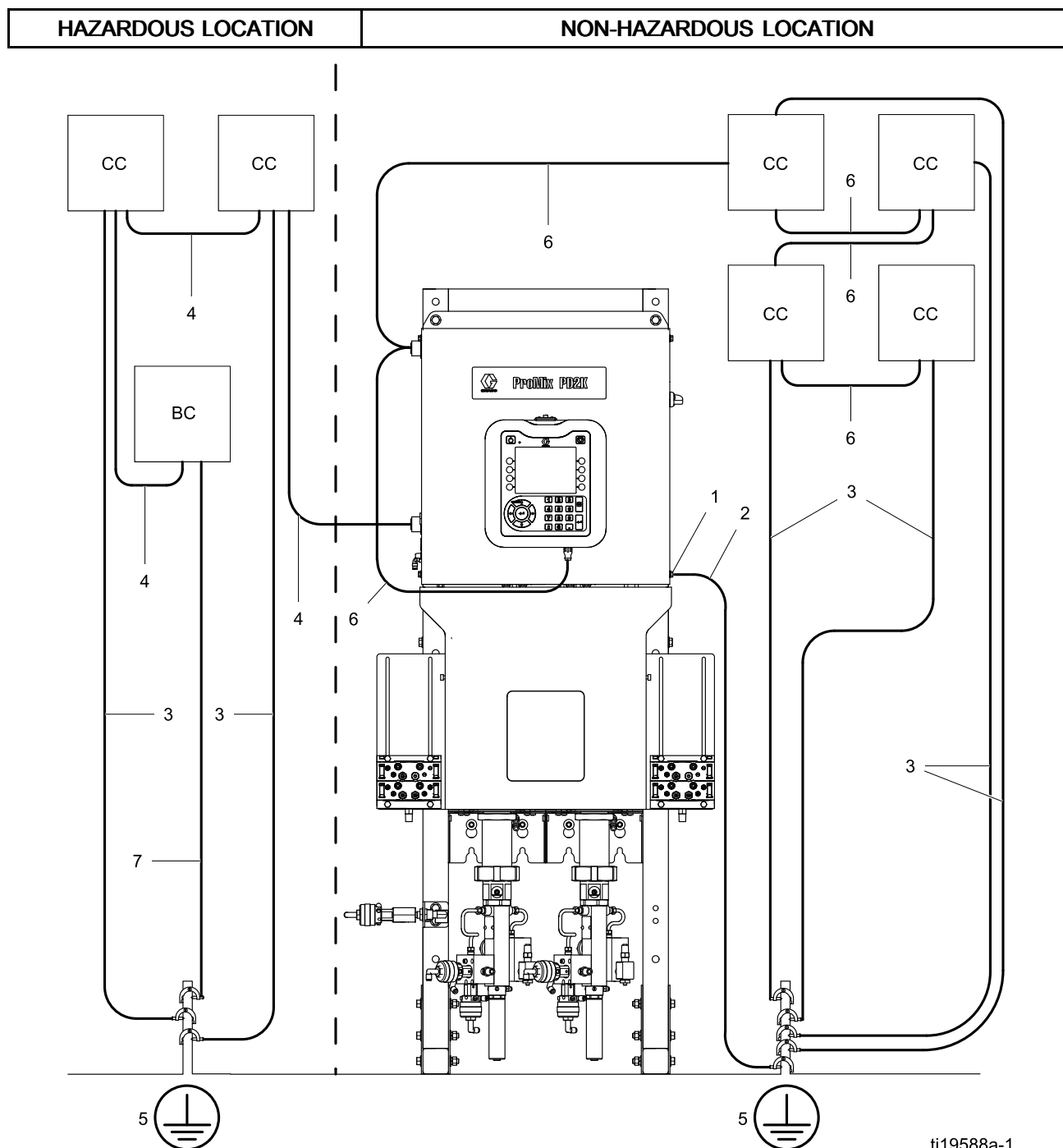
Figure 23 System Grounding
