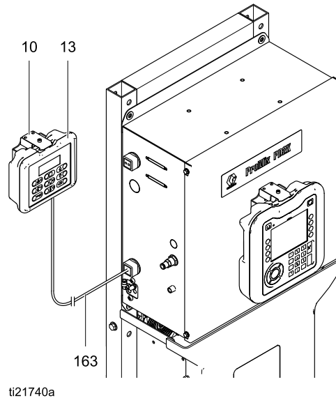
Figure 15 Install the Booth Control
