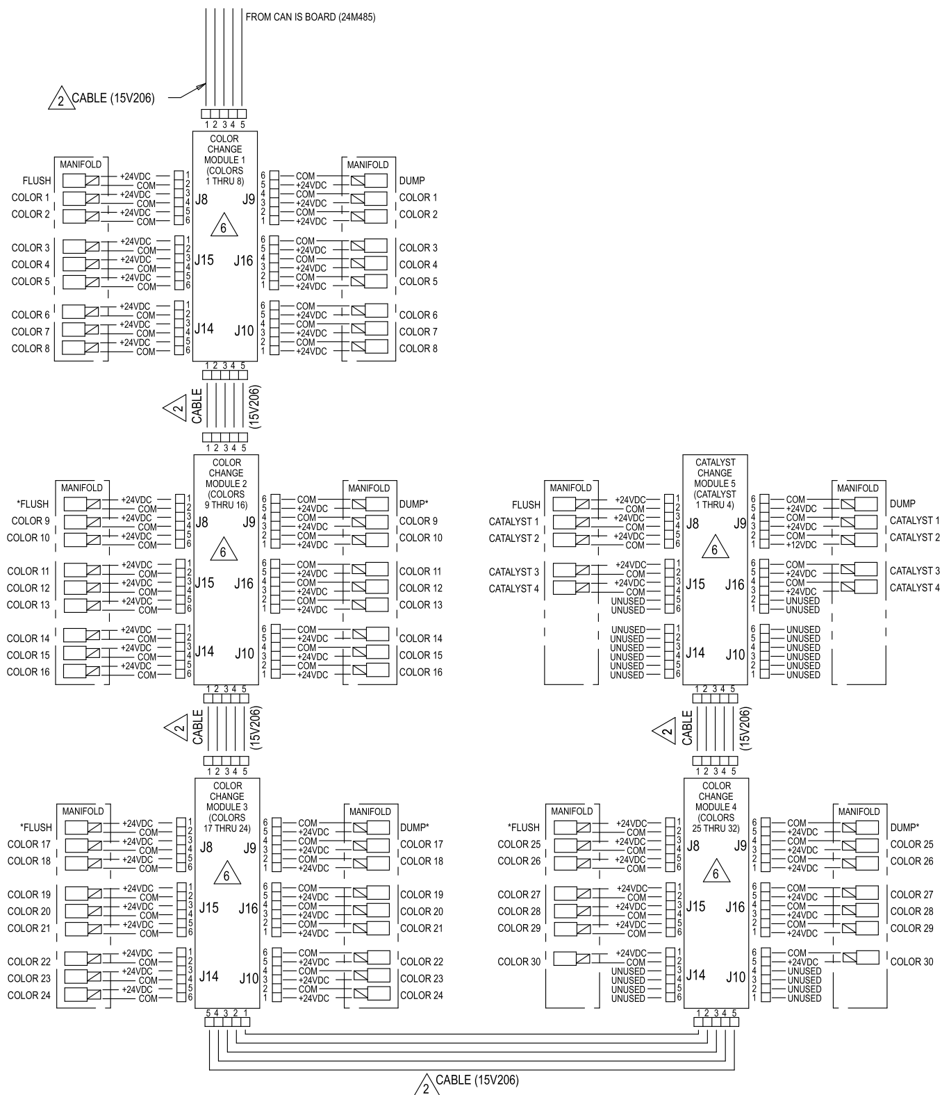
Figure 33 Electrical Schematic, Sheet 3, Part 1
