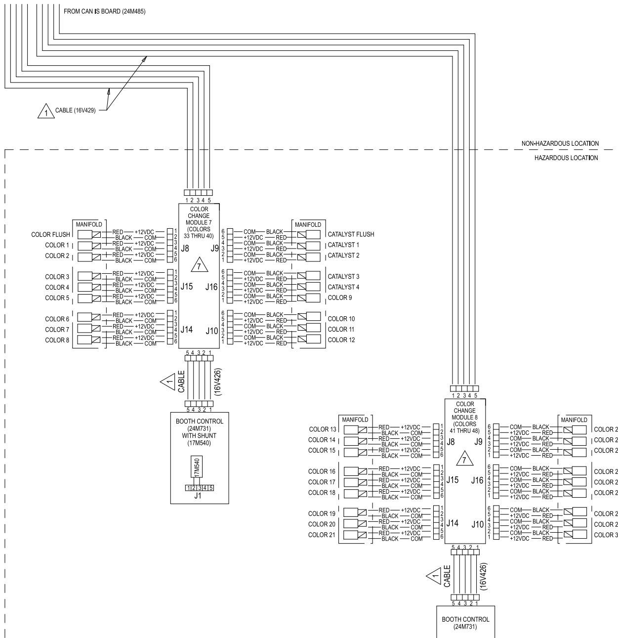
Figure 34 Electrical Schematic, Sheet 3, Part 2
