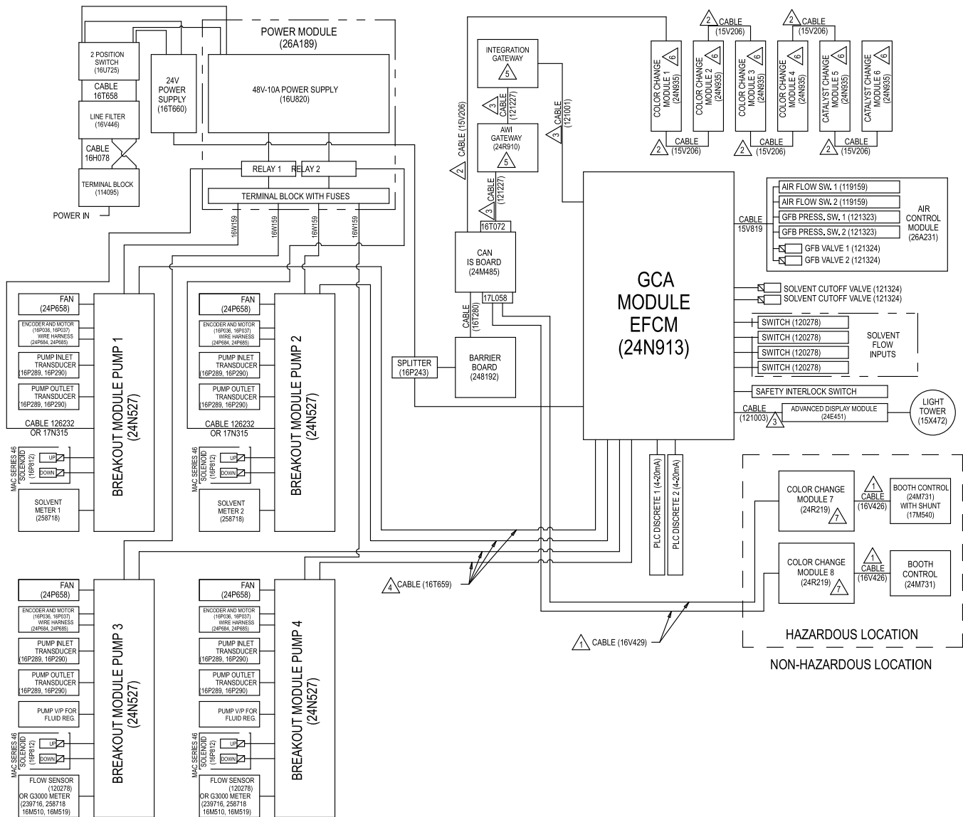
Figure 30 Electrical Schematic, Sheet 1
