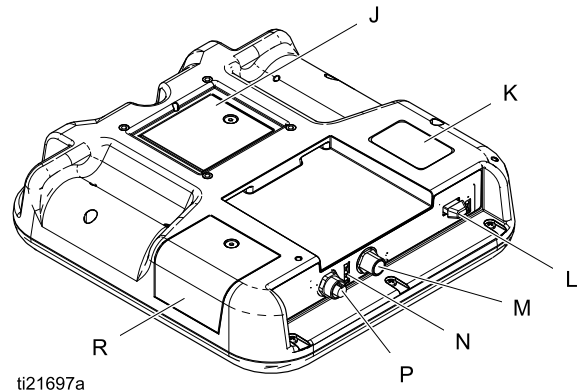
Figure 13 Advanced Display Module Connection Ports
