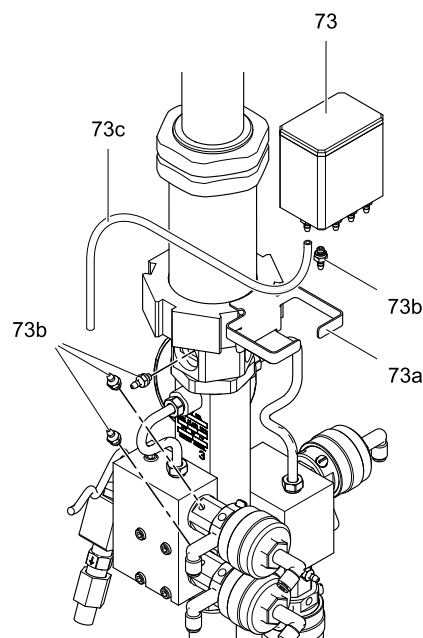
Figure 19 Install TSL Cup Kit
