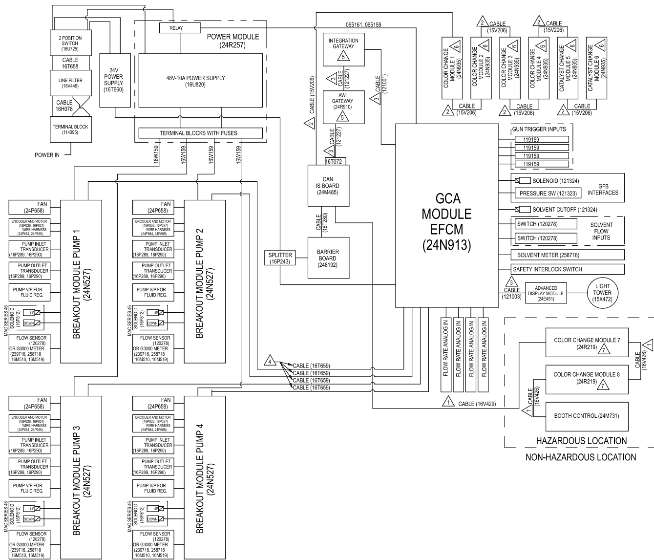
Figure 24 Electrical Schematic, Sheet 1
