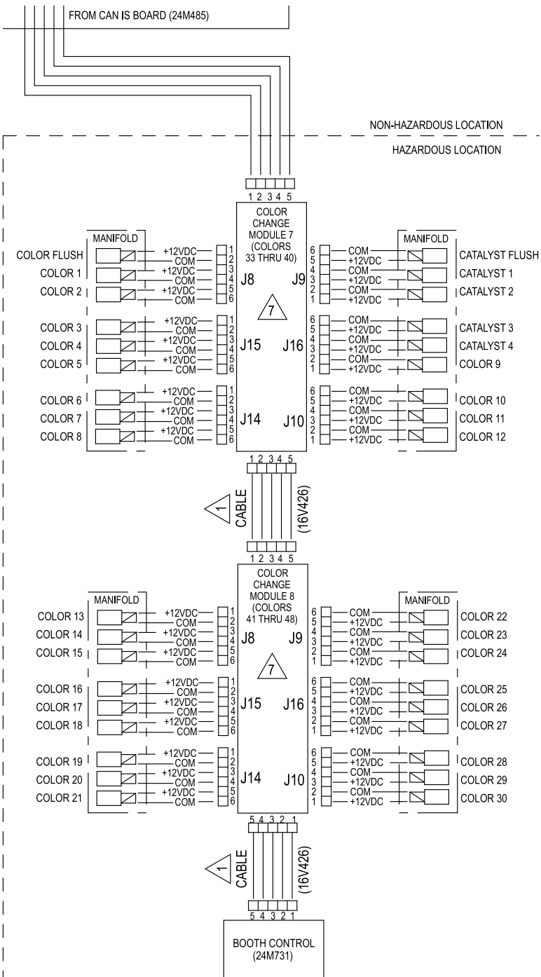
Figure 29 Electrical Schematic, Sheet 3, Hazardous Location
