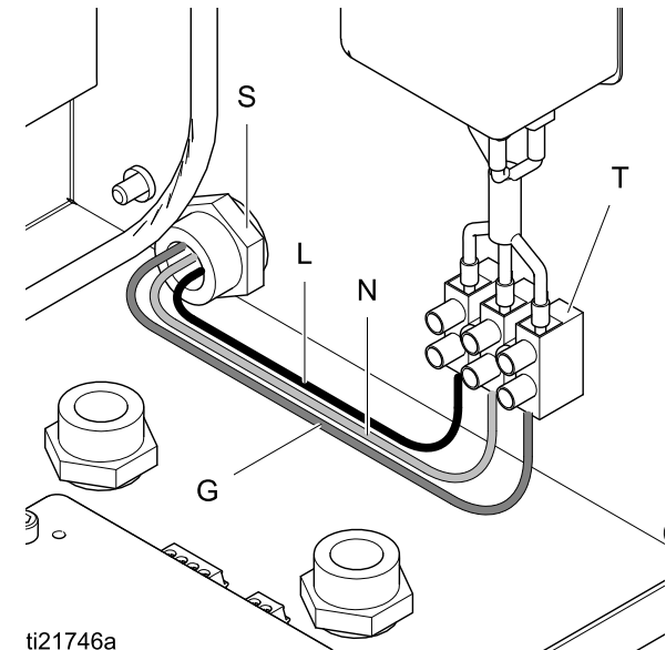
Figure 21 Control Box Electrical Connection
