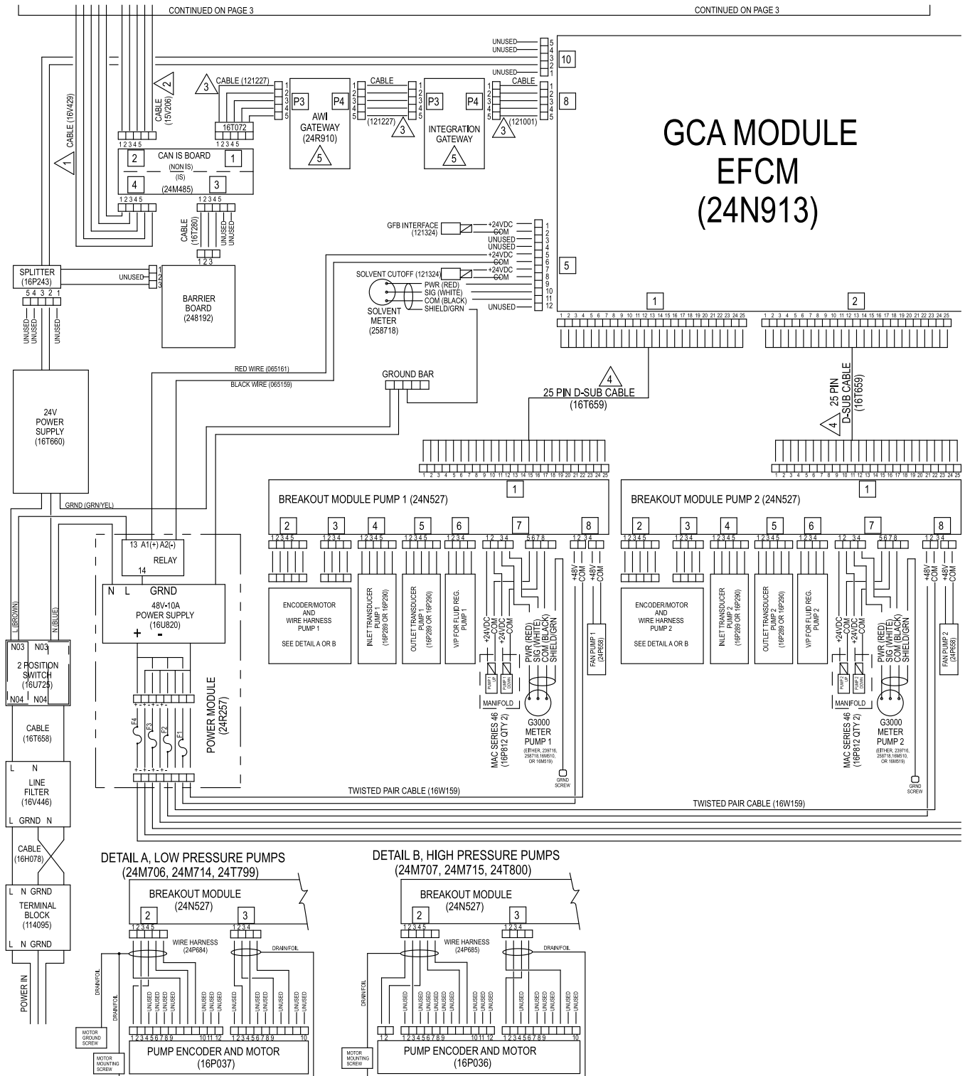
Figure 25 Electrical Schematic, Sheet 2, Part 1
