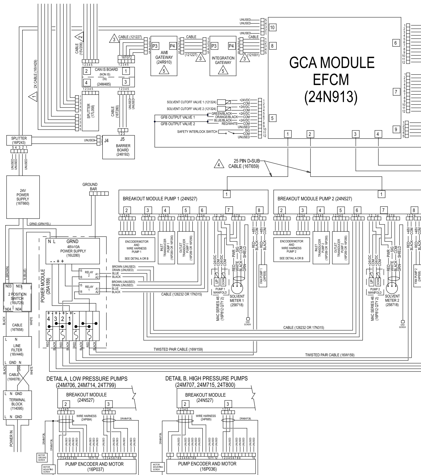
Figure 31 Electrical Schematic, Sheet 2, Part 1
