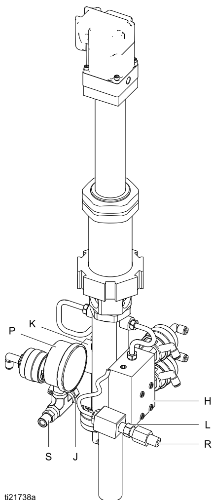
Figure 18 Pump Inlet and Outlet Connections
