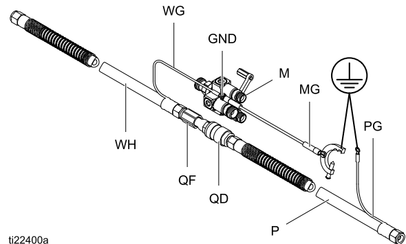
Figure 20 Electrostatic Air Hose Quick Disconnect Kit
