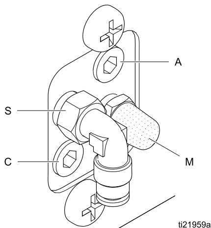
Figure 17 Air Manifold Connections
