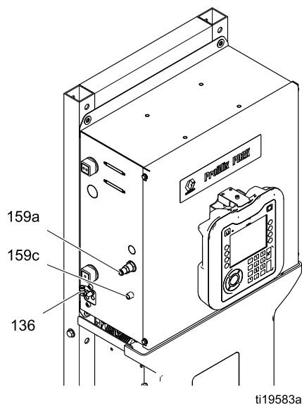
Figure 16 Connect Atomizing Air
