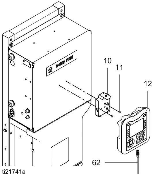
Figure 12 Install Display Module
