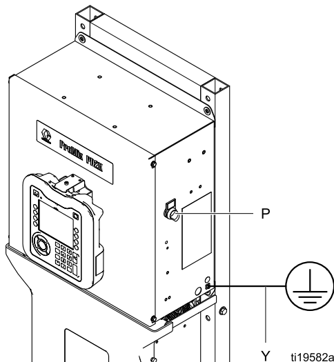
Figure 22 Ground Screw and Power Switch
