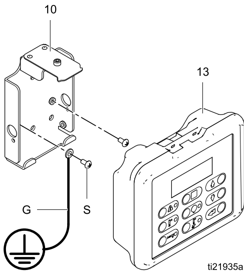
Figure 14 Ground the Booth Control Bracket
