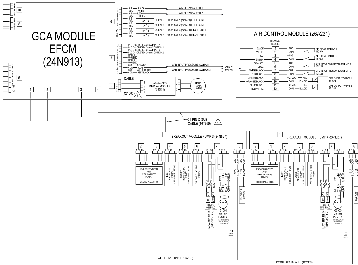
Figure 32 Electrical Schematic, Sheet 2, Part 2
