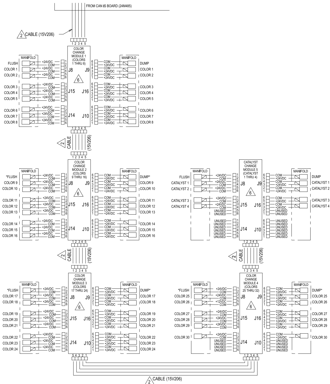
Figure 27 Electrical Schematic, Sheet 3
