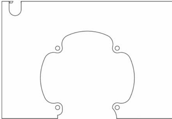
247312 Adapter Plate (required to mount NXT 2200 Air Motor to 255143 Bracket)
