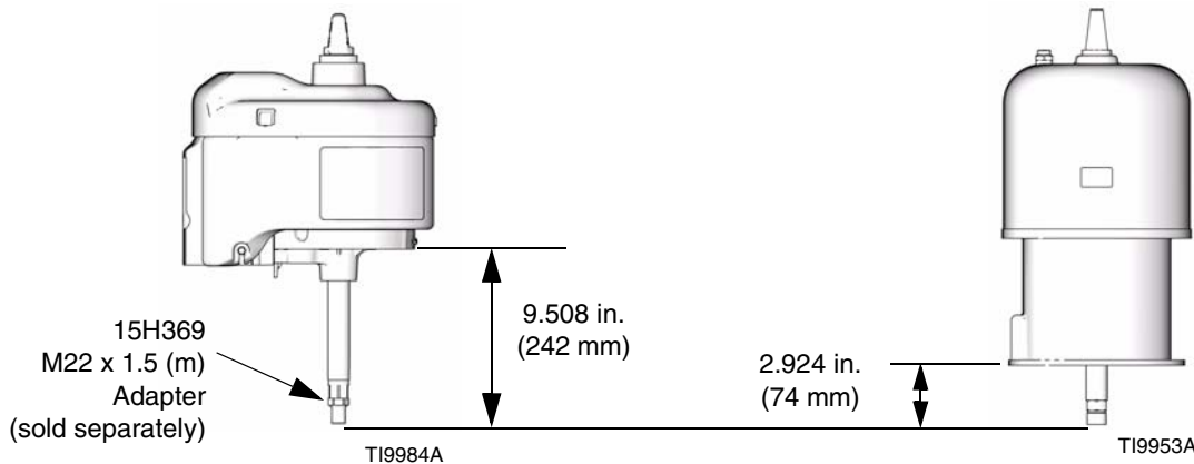
NXT Motor with Small High-Flo Pumps
