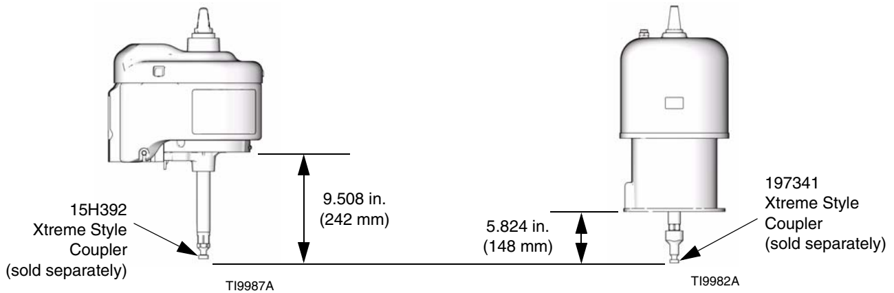
FIG. 5. Dimensions for Xtreme Pumps
