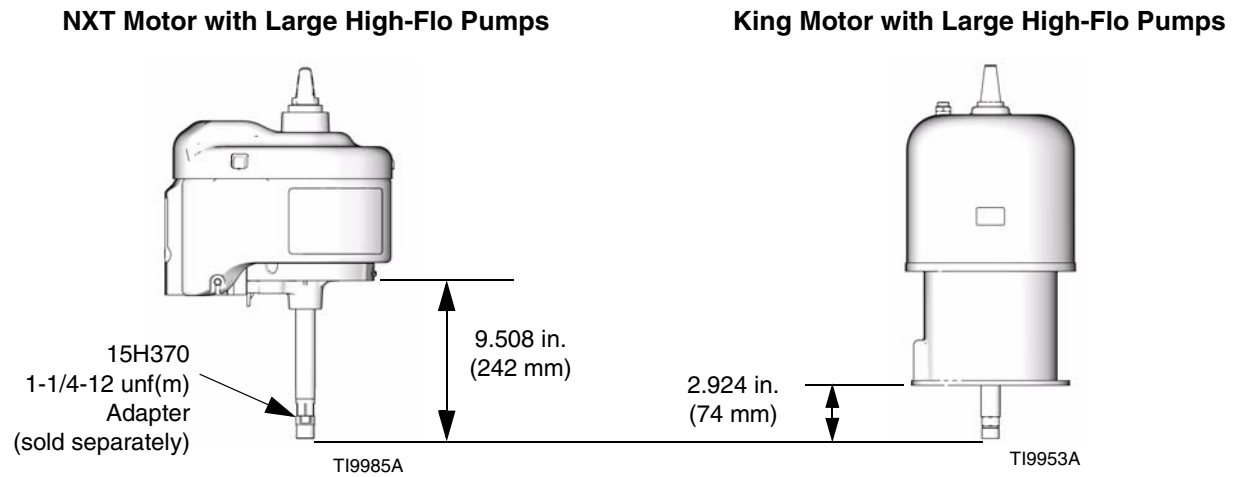
FIG. 2. Dimensions for Large High-Flo Pumps
