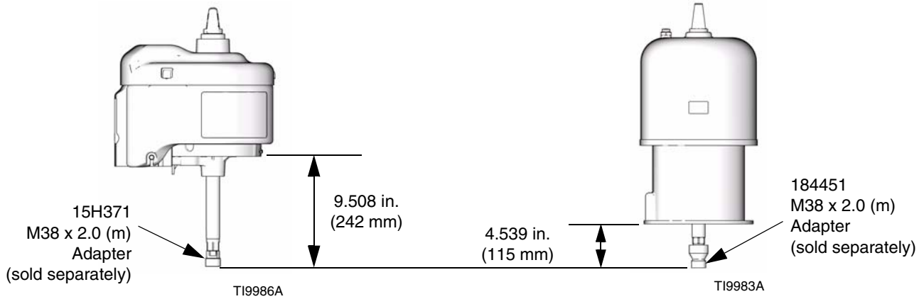
FIG. 4. Dimensions for Dura-Flo 1800-2400 Pumps
