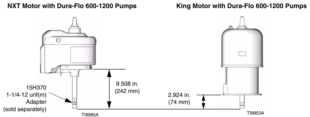
FIG. 3. Dimensions for Dura-Flo 600-1200 Pumps
