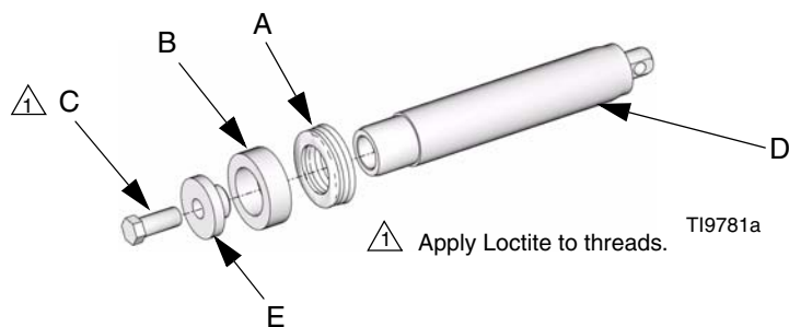
FIG. 1: Piston Seal Kits
