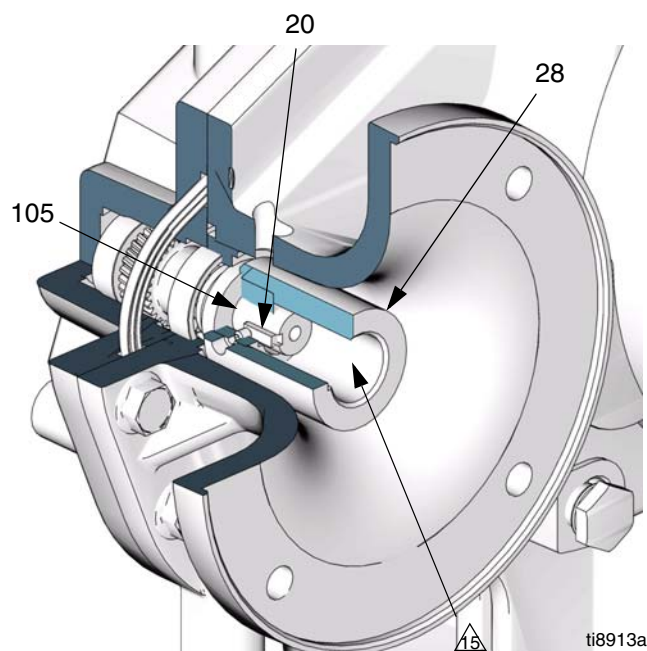
FIG. 4. Motor Coupler Installation
