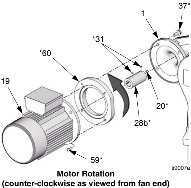
FIG. 2. IEC 112M/B5 Frame Electric Motors
