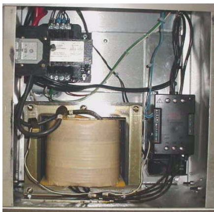
FIG. 4: Completed Installation - H-20/35 Pro
