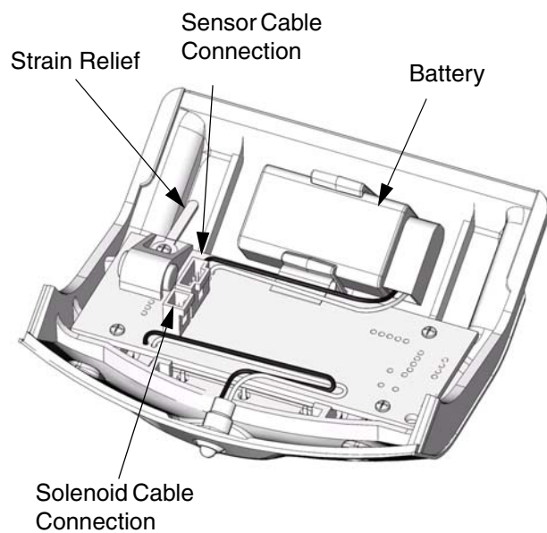
FIG. 1. Battery Location and Module Cable Connections
