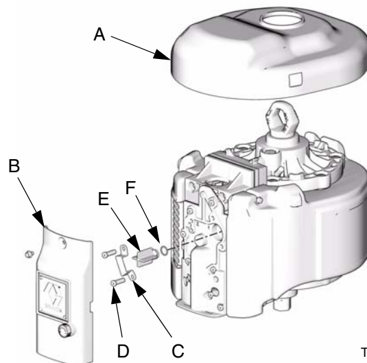
FIG. 2. Disassembly
