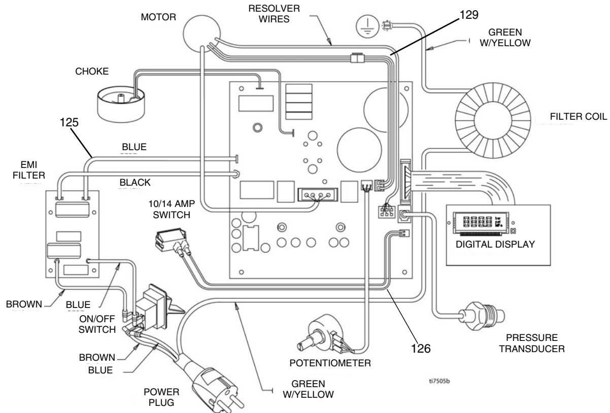
WIRING DIAGRAM
