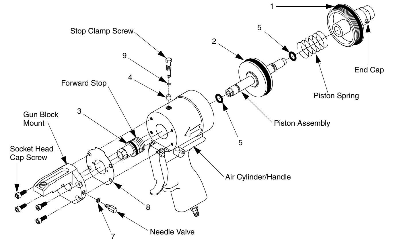
FIG. 3: Kit 296895 for GX-7, GX-7 400, and GX-7 DI Conversion Spray Guns
