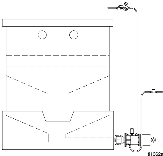
Horizontal Mount
