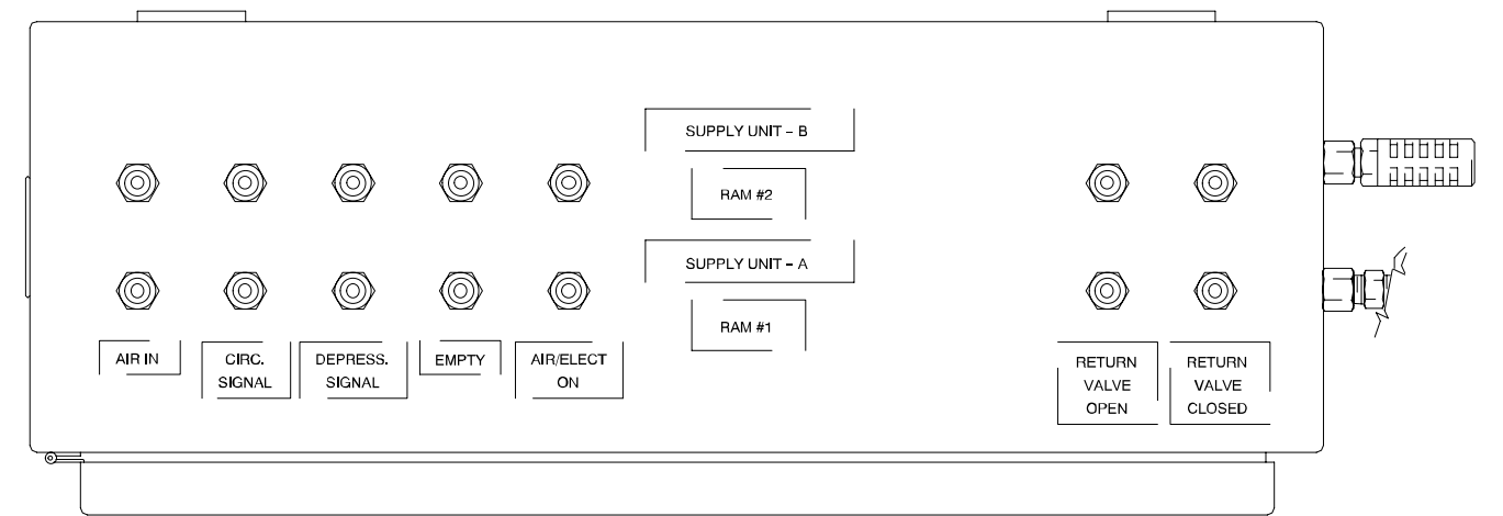
Timer/Pneumatic Interface – Top View
