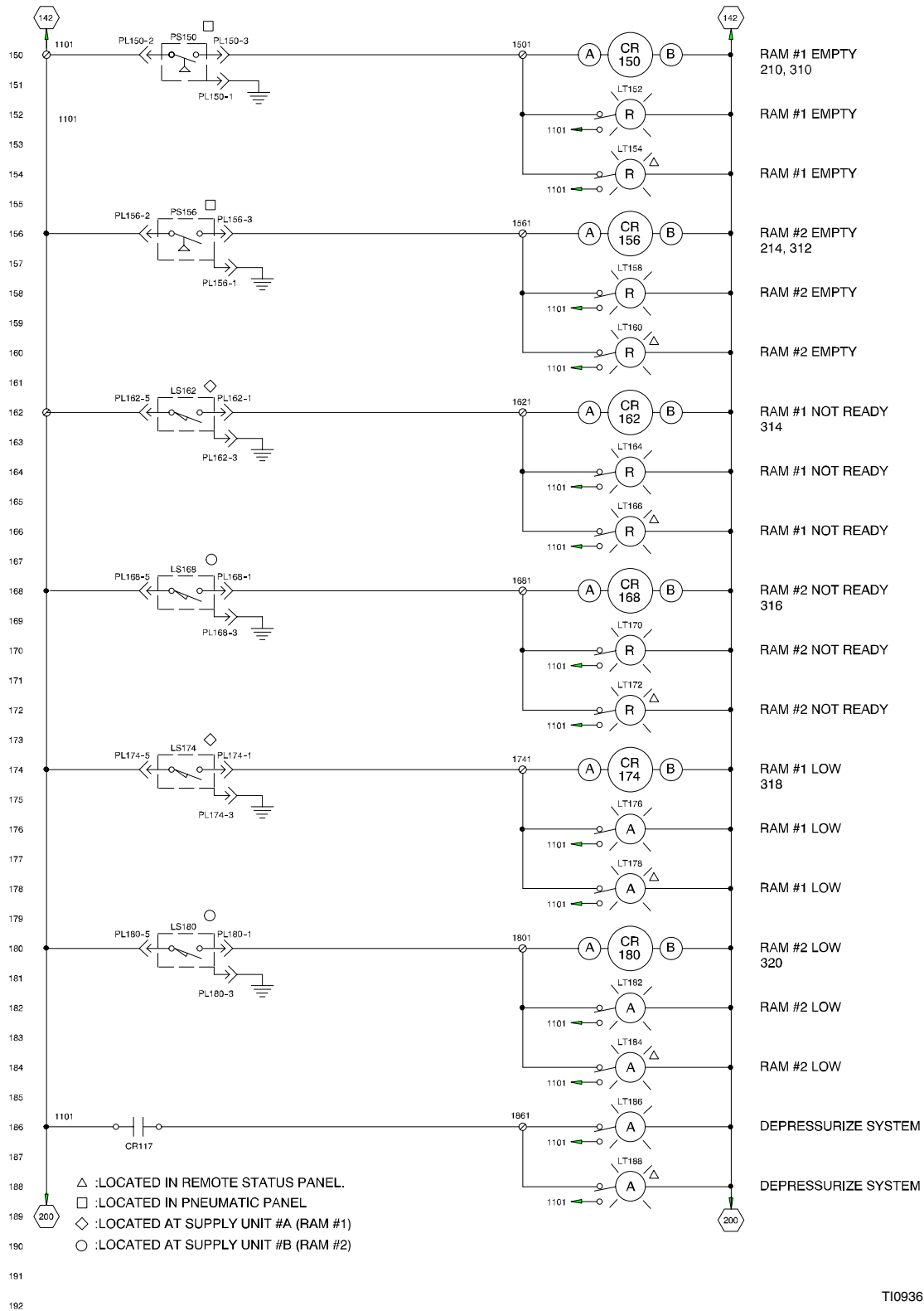
7-Day Timer Wiring Diagram (Sheet 2 of 4)
