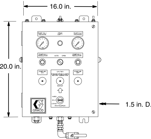
243559 Pneumatic Control
