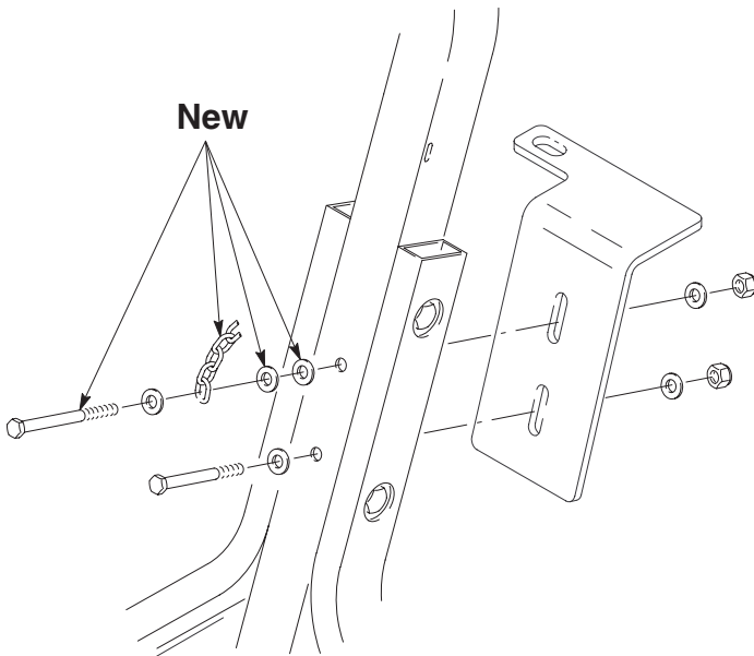
2. Reassemble plate as shown
