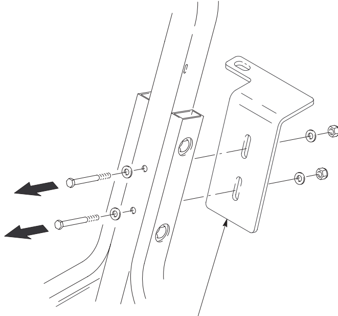
3. Remove and inspect plate for cracks (Replace as needed)
