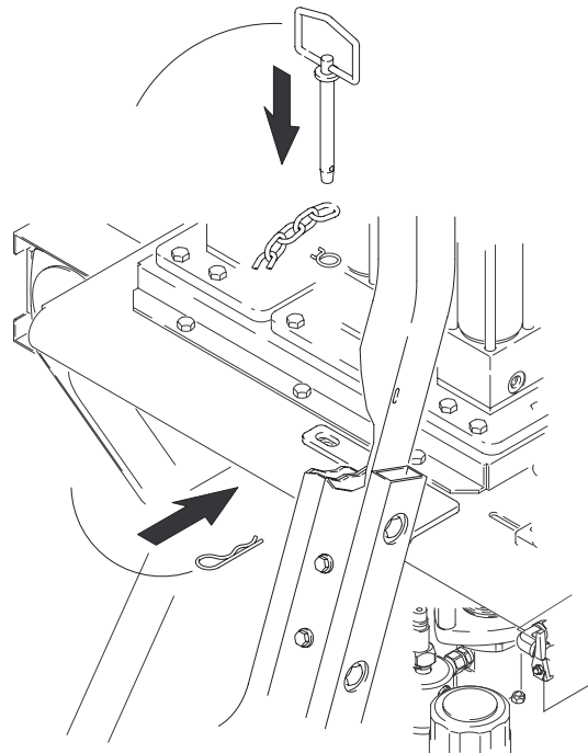
4. Install new pin
