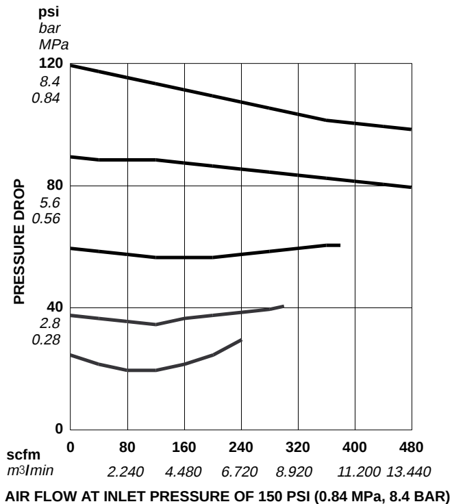
MODEL 114–459 AIR REGULATOR FLOW CURVE
