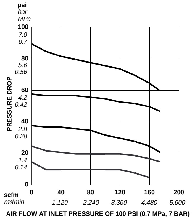
MODEL 114–105 AIR REGULATOR FLOW CURVE
