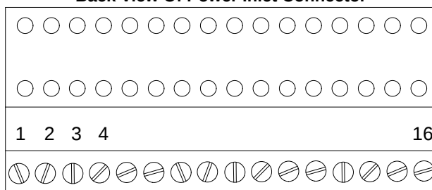
Back View Of Power Inlet Connector
