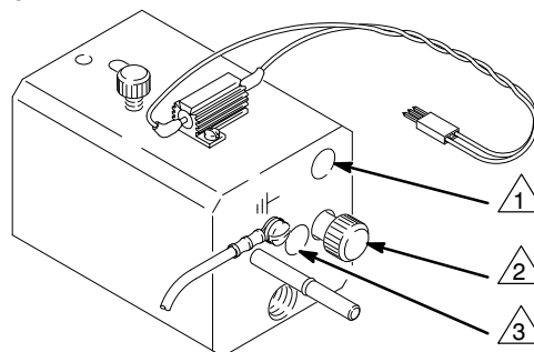
Back View of PRO ES Test Fixture
