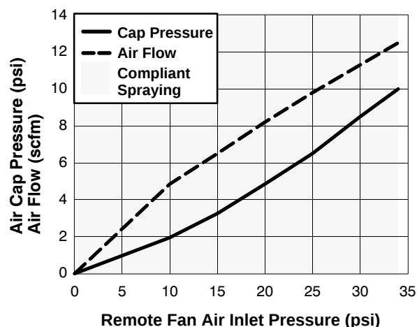
Horn Pressure and Air Flow
