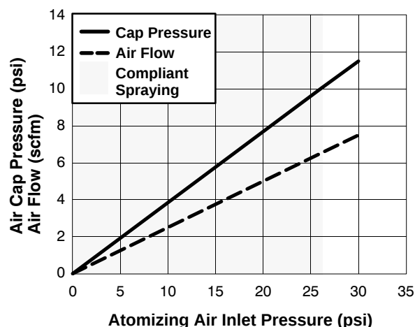
Atomization Pressure and Air Flow
