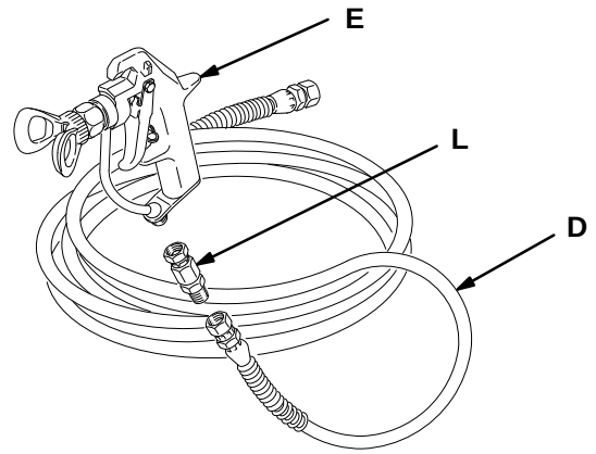
DETAIL B: ASSEMBLY OF HOSE AND GUN (MODELS 224-625 AND 231-163)
