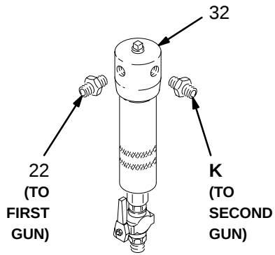
DETAIL A: HOSE CONNECTIONS AT FLUID FILTER (ALL MODELS)
