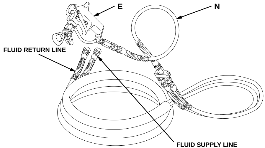
DETAIL D: ASSEMBLY OF HOSE KIT AND GUN (MODELS 224-630 AND 231-160)
