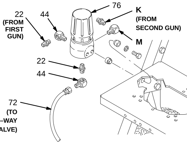
DETAIL C: FLUID RETURN CONNECTIONS AT BACK PRESSURE VALVE (MODELS 224-630 AND 231-160 ONLY)
