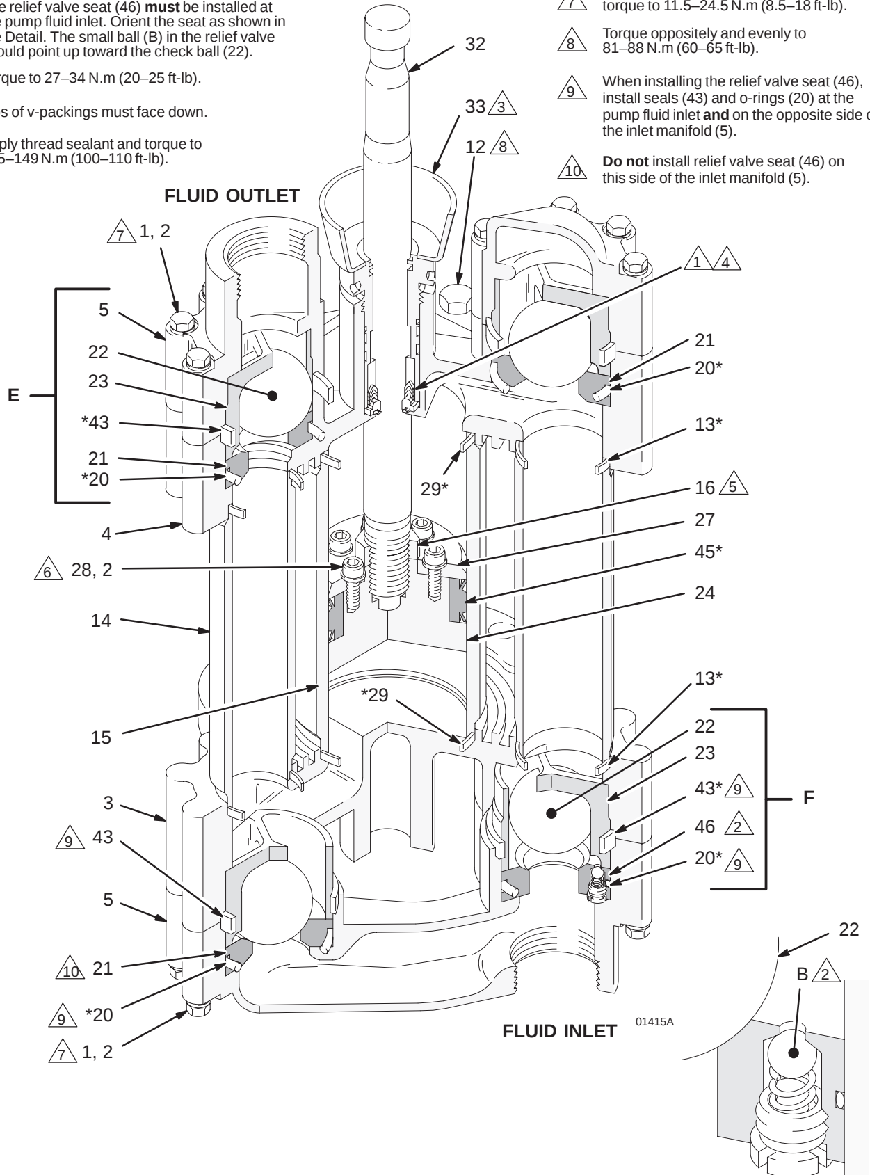
Detail of Inlet Valve Seat (46)
