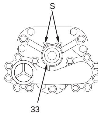
Top View of Displacement Pump (Stainless Steel Pump Shown)
