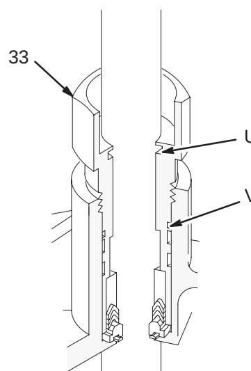
Installing O-Rings on Packing Nut (Carbon Steel Pumps)
