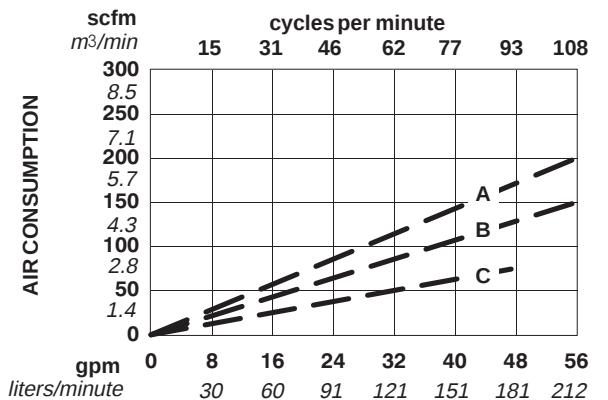
Air Consumption
