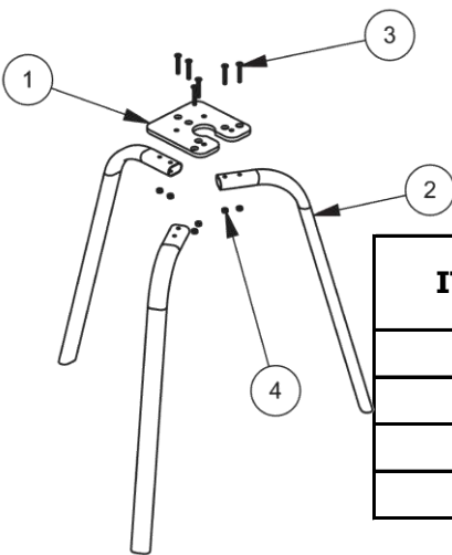
0115-010100 TRIPOD
